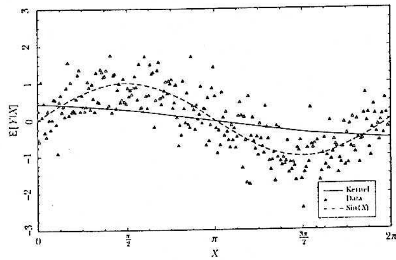
(c) h = 0.5\hat{\sigma}_x
