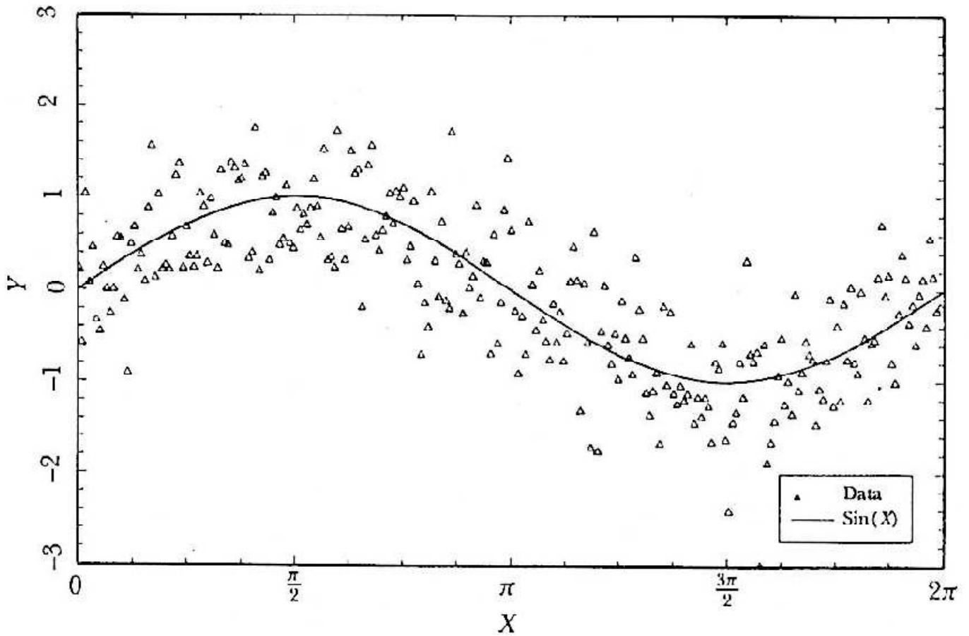
Figure 12.4. Simulation of Y_t = \sin(X_t) + 0.5\epsilon_t
