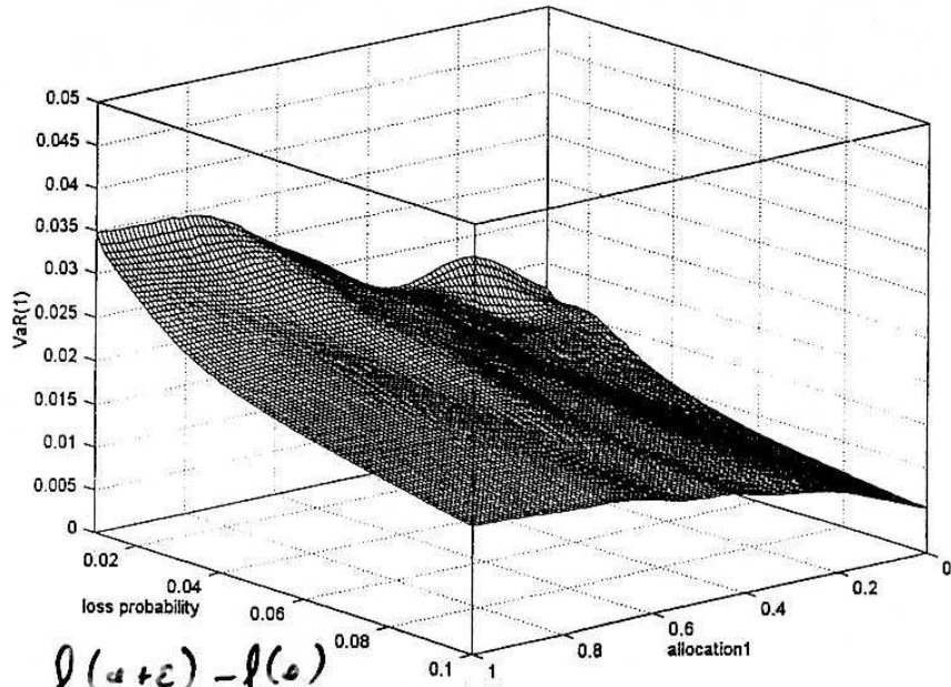
Gaussian kernel VaR sensitivity estimation wrt a1
