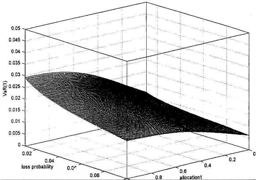
Gaussian assumption VaR sensitivity wrt a1
