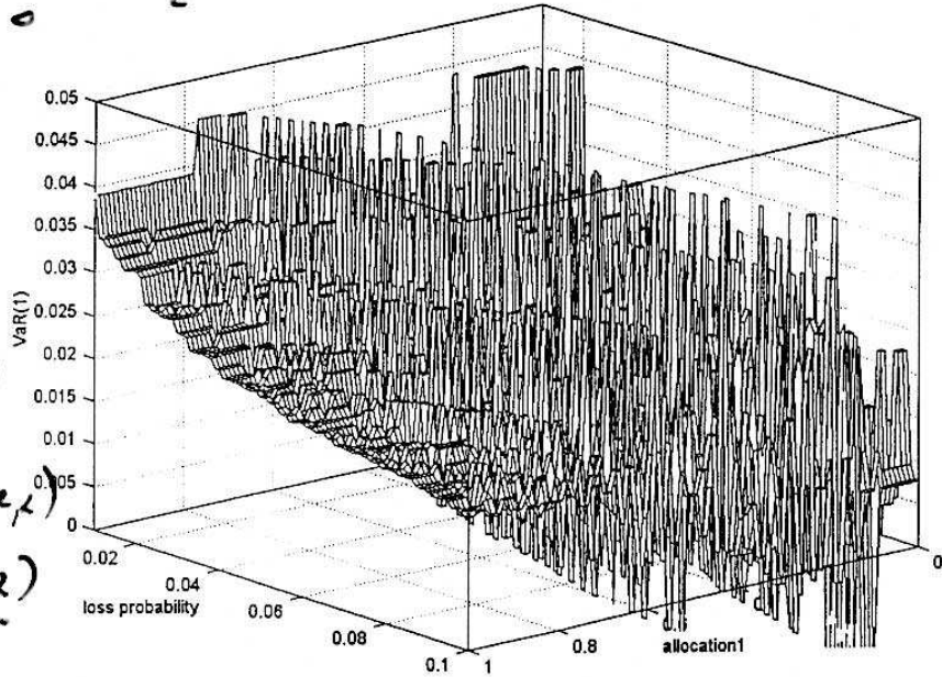
Gaussian assumption VaR sensitivity wrt a1
